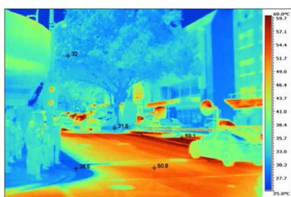
A thermal image at the corner of Russell and Bourke Streets, when the day's top temperature was 32.4. Numbers on this photo indicate degrees Celsius. (Photograph: Jason Dowling, courtesy City of Melbourne)
